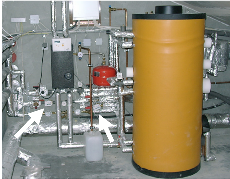
Figure 41: Installation wall on the building services floor with water storage tank. The two heat quantity meters are marked with arrows.
