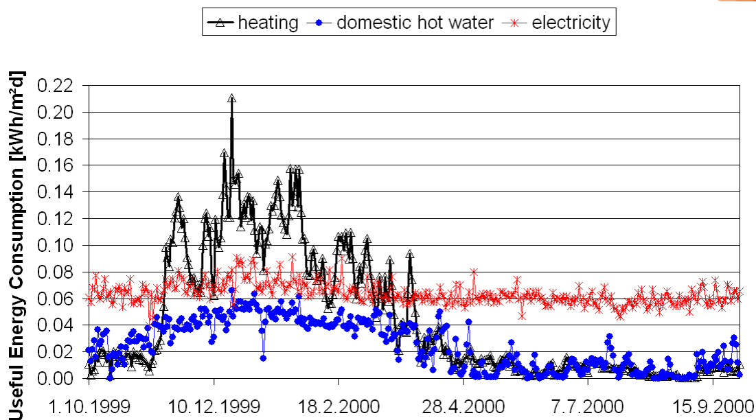
Figure 47: Energy consumption per day in the permanently occupied houses in the first measurement year
