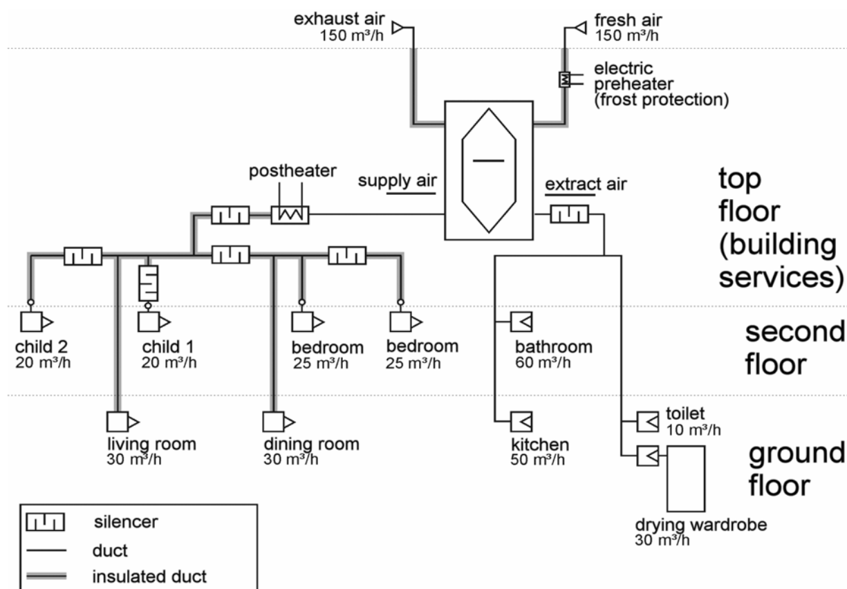
Figure 18: Ventilation system duct network plan for Passive House type „Jangster de L  x“ with the design layout flow volumes
