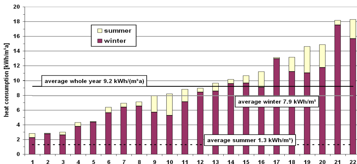
Figure 68: Specific district heating consumption for domestic hot water preparation during the first measurement year (01.10.1999 to 30.09.2000) for the 22 permanently occupied Passive Houses divided in winter (01.10.1999 to 30.04.2000) and summer period (01.05.2000 to 30.09.2000).
