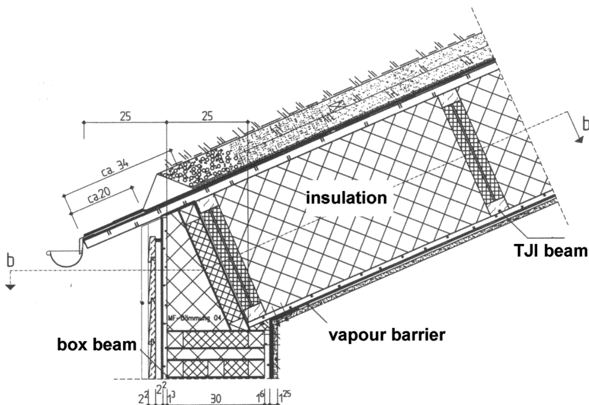
Figure 11: Thermal-bridge-free eaves junction of the roof element to the facade element
