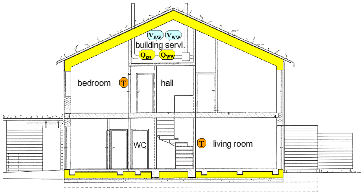
Figure 39: Cut-away section through a terraced Passive House with drawn-in location of the measurement points for the standard measurement (according to [Pfluger 2000]).
