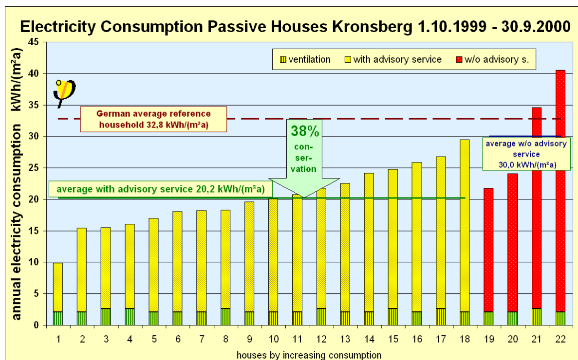
Figure 71: Measured annual electricity consumption of the 22 Passive Houses (permanently occupied in 1999/2000) from 1.10.1999 to 30.09.2000 (household, auxiliary and ventilation electricity, but without common electricity).
