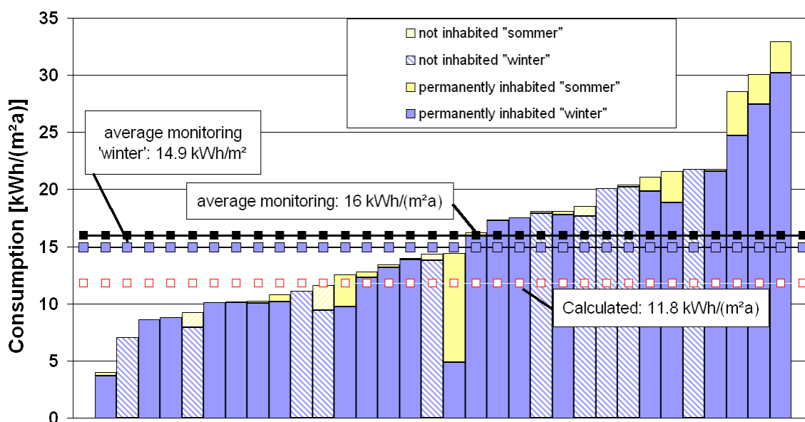
Figure 48: Comparison of the measured heating consumption and the projected (calculated) heating consumption values in the first year of measurement (1.10.1999 to 30.9.2000).
