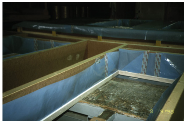
Figure 30 (left): Facade element window opening. The airtight foil joints are carefully glued, the overhanging foil is there to allow for an airtight seal with the next elements
