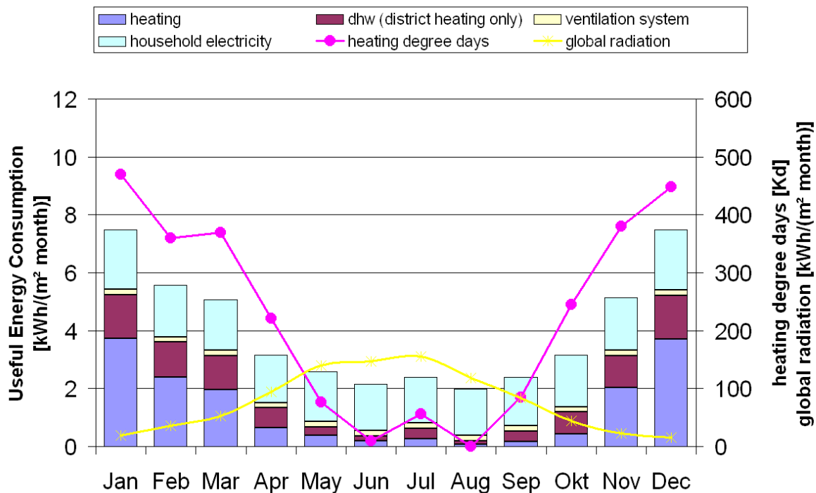
Figure 46: Monthly energy requirement for the permanently occupied Passive houses in the first measurement year (01.10.1999 to 30.09.2000).
