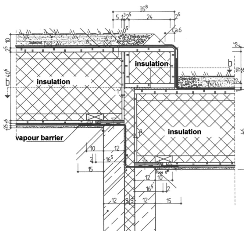
Figure 8: Thermal-bridge-free junction of two offset roof elements
