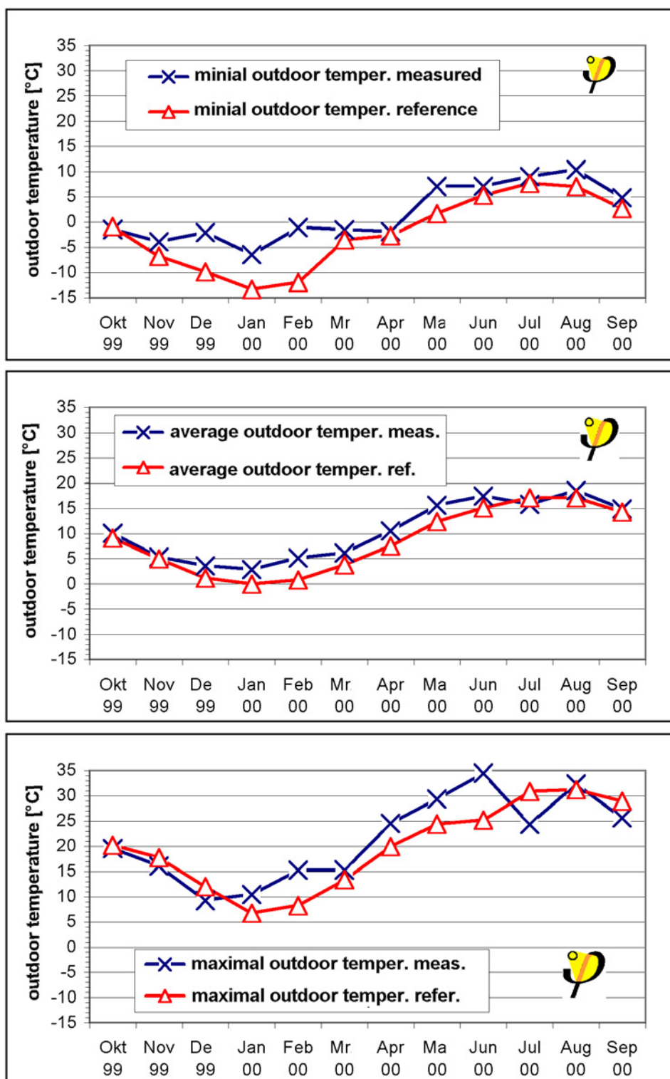
Figure 65: First measurement year climate data comparison of the minimal, average and maximum temperatures (monthly values from hourly data) between the measurement data and the reference data, which are used for the simulation [Schnieders 98].
